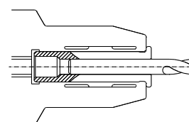
Croquis HSK-A/WD-CB
