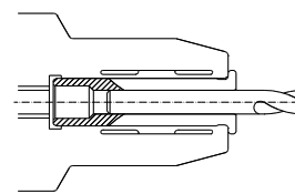
Drawing HSK-A/WD-CB
