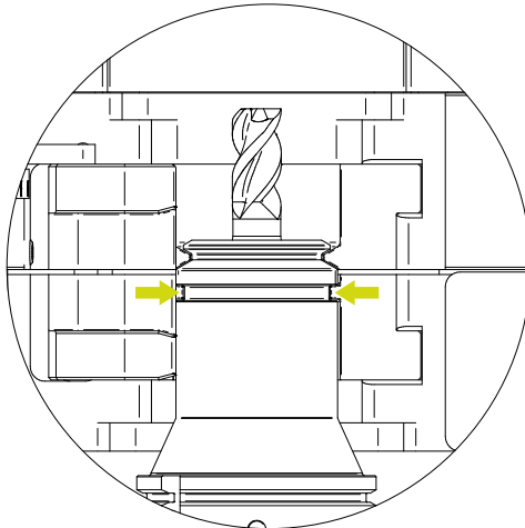
Figure 3.2b Position d'insertion Extraction.
