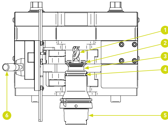
Figure 3.2a Position d'insertion Insertion.
