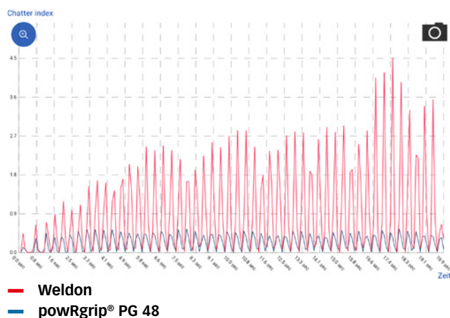
Vibrations on the workpiece (Detected and visualized using REGO-FIX toolVibe®)
