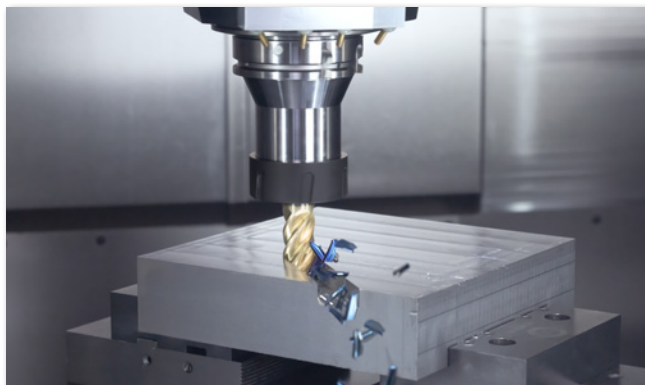
Vibrations on the spindle (Detected and visualized using REGO-FIX toolVibe®)
