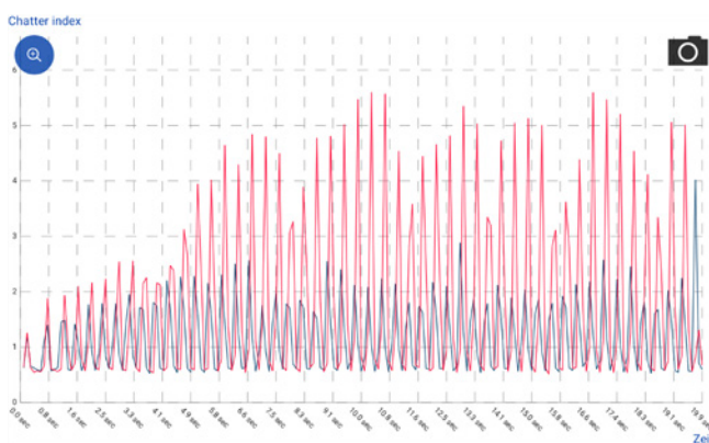
Vibrations on the spindle (Detected and visualized using REGO-FIX toolVibe®)
