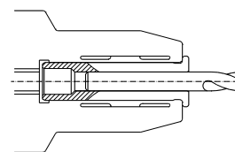
Drawing 1 HSK-A/WD
